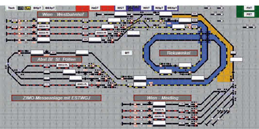
The ESTWGI interlocking for the ZIMO N-gauge layout: The purely technical demo layout is 2 x 1.3 m big, includes 3 stations with a total of 14 tracks, 3 routes with block operation and 1 reversing loop. The electronic equipment consists of an MX10 command station with (usually) at least 2 cabs (currently MX33), and 8 StEin modules; there are special ones for the signal bridges, some with integrated accessory decoders MX820, partly with modified StEin signal boards.
