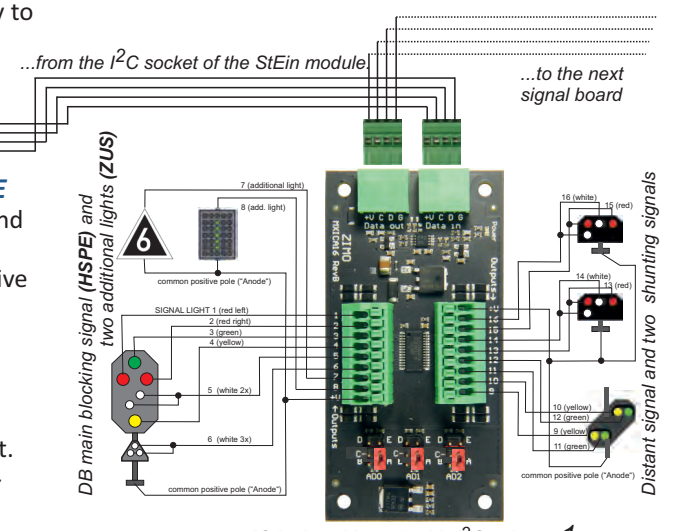
ICA signal board with I2C address 1
